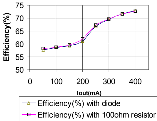
Efficiency versus load current
