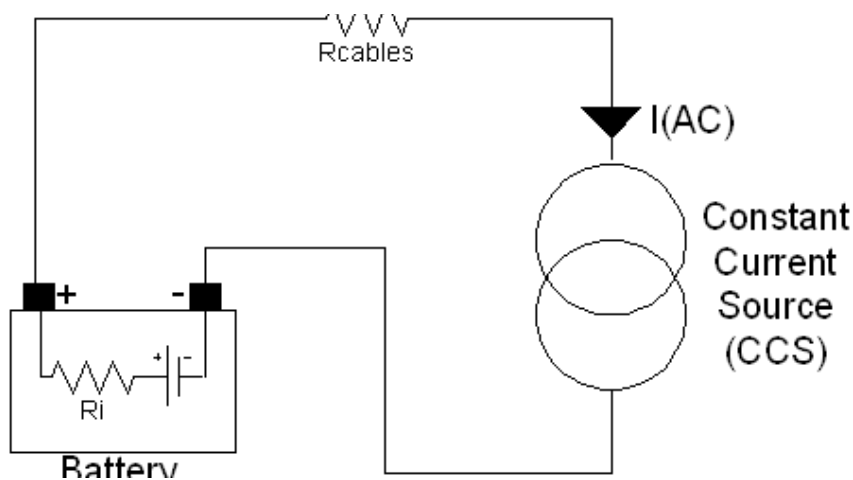
Figure 7. Internal resistance measurement
