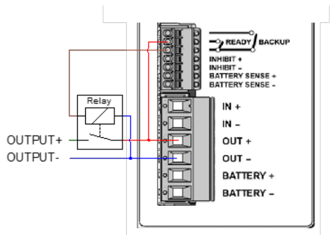
Figure 4. External relay
